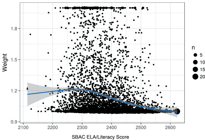
Figure 2. Illustration of relationship between SBAC ELA/literacy scores and probability of membership in confusion class (Weight), grade 3, CORE SEL data (sample of 5,000 students).
