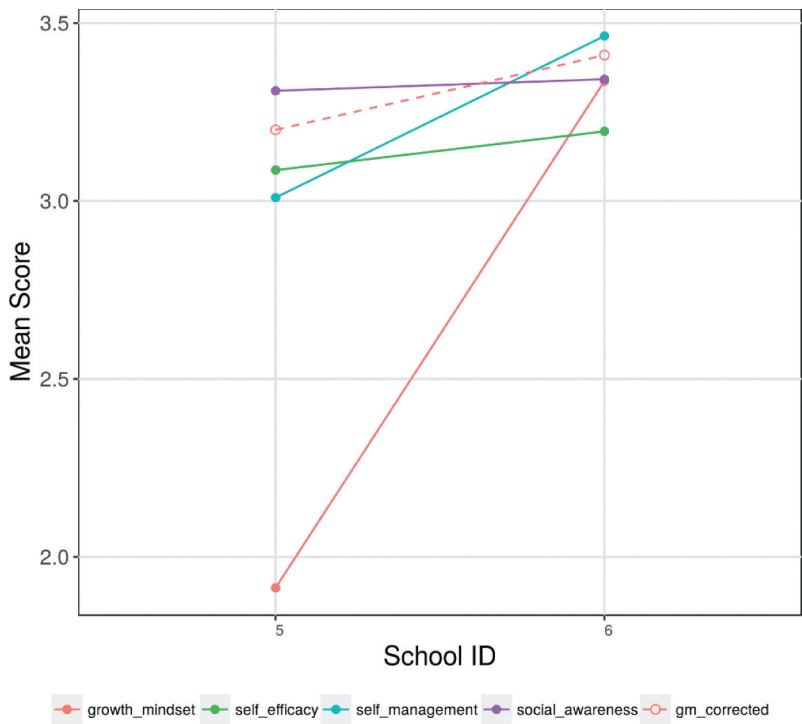
Figure 4. Illustration of effects of school-level correction of GM scores due to confusion, two schools (5&6), CORE SEL data, grade 3.
