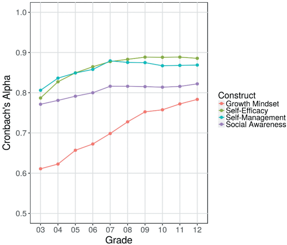
Figure 1. Cronbach alpha estimates by SEL construct, grades 3–12, CORE districts.
