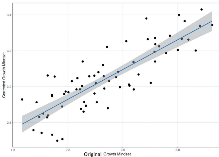
Figure 3. Illustration of effects of student and school-level correction of GM scores due to confusion, CORE SEL data, grade 3. (a) Scatterplot of original and corrected student GM scores (b) Scatterplot of original and corrected school-level GM scores.
